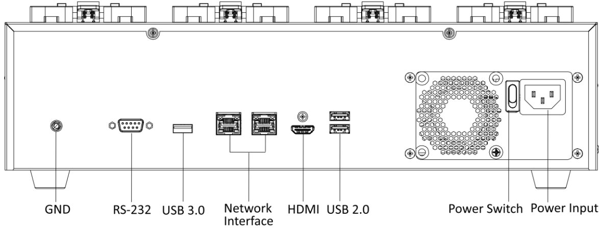
Figure 1-3 Rear View 2
