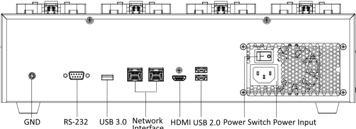
Figure 1-2 Rear View 1
