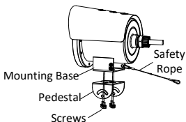
Figure 1-8 Fix the Camera to the Pedestal
