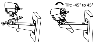
Figure 1-10 Secure the Camera to Wall Mounting Bracket
