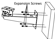
Figure 1-6 Install the Wall Mounting Bracket
