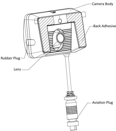
Figure 1-1 Overview
