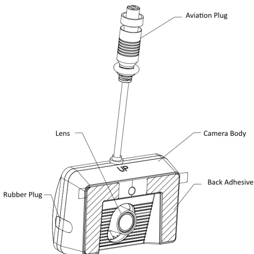
Figure 1-4 Top Wiring
