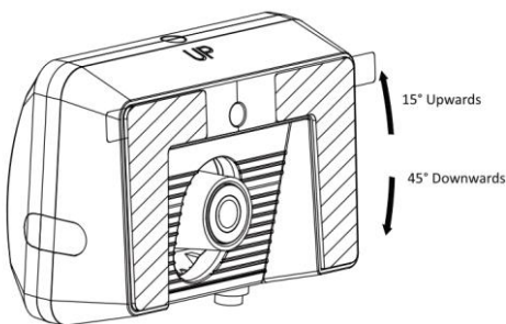
Figure 2-5 Range for Angle Adjustment
