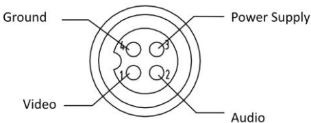
Figure 1-3 B Sequence
