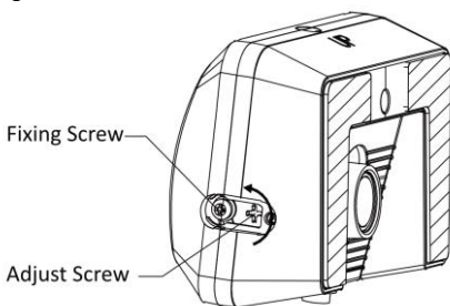
Figure 2-4 Adjust the Angle
